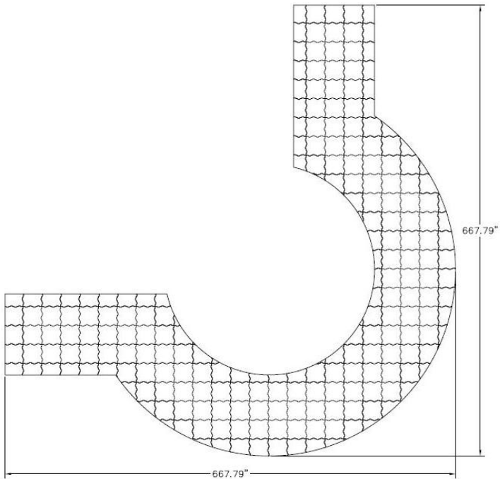
#185U 10' With Wings Panel Assembly 02/28/12
