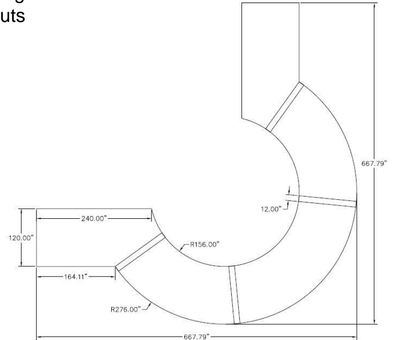
#185U 10' With Wings Turf Assembly * 02/28/12
