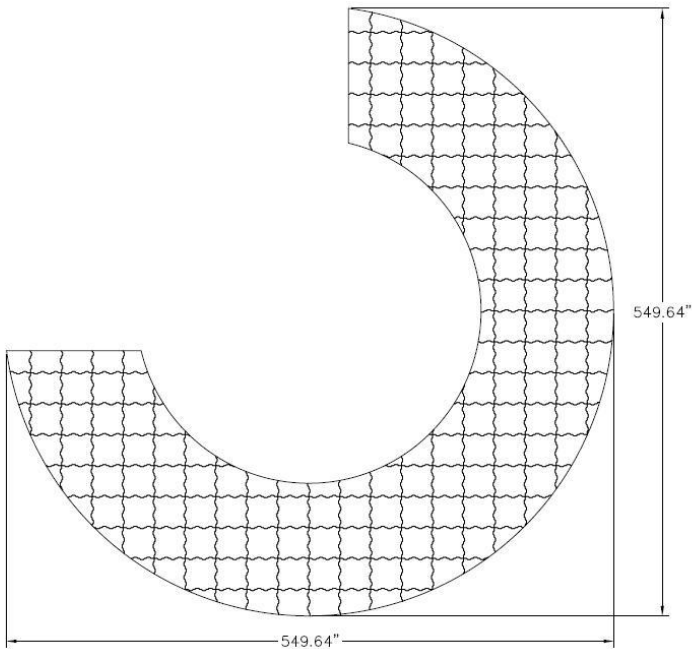
#185U 10' No Wings Panel Assembly 03/04/12
