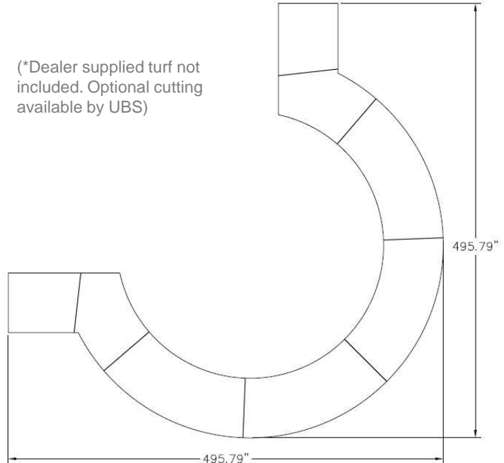
#185U 5' With Wings Turf Assembly* 03/11/12
