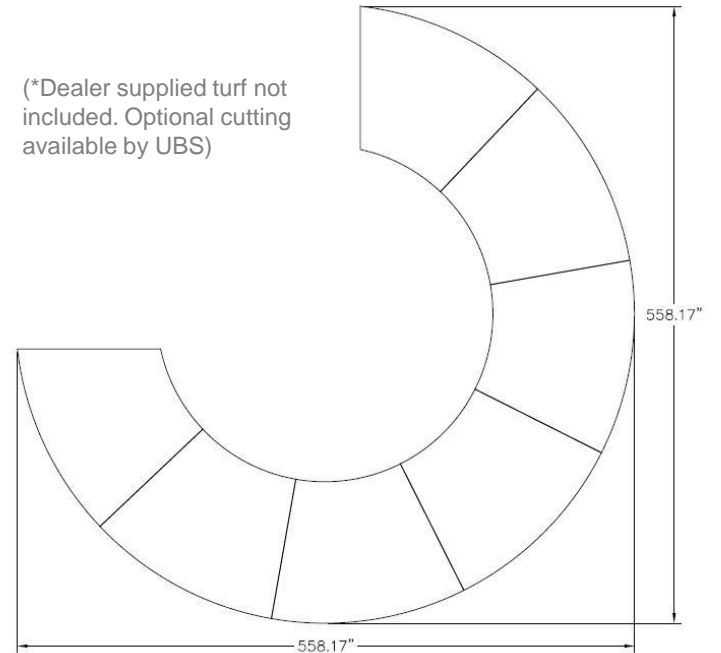
#185U 10' No Wings Turf Assembly * 03/04/12
