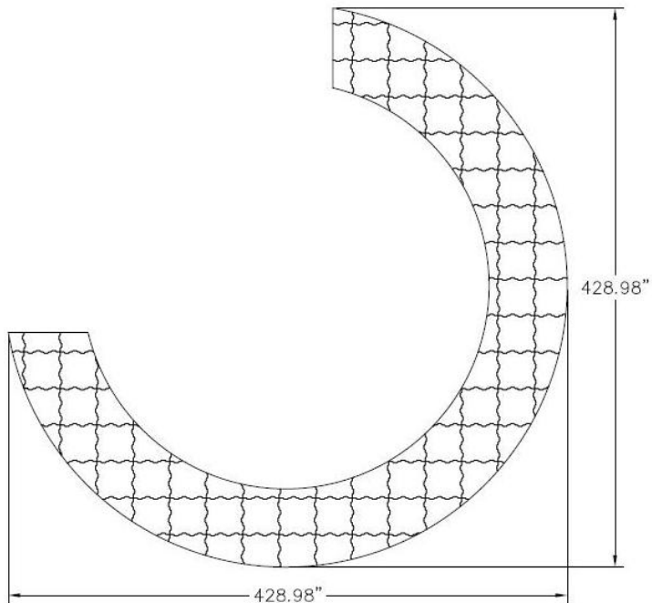
#185U 5' No Wings Panel Assembly 03/07/12
