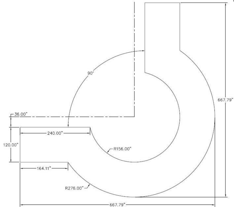
#185U 10' With Wings Panel Assembly 02/28/12
