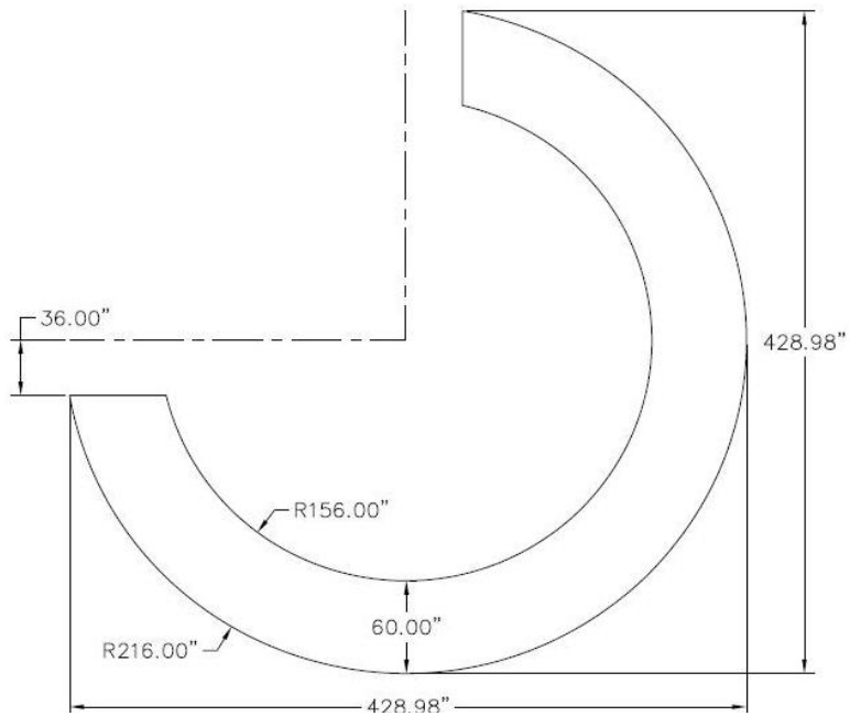
#185U 5' No Wings Panel Assembly 03/07/12
