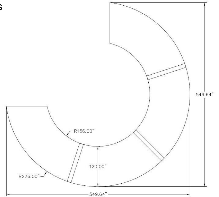
#185U 10' No Wings Turf Assembly * 03/04/12
