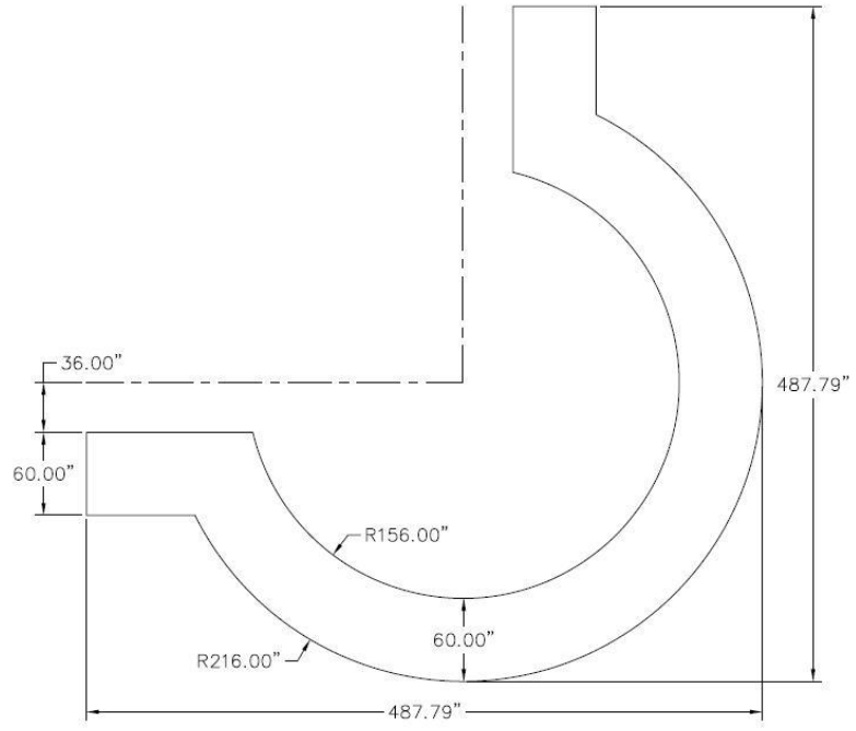
#185U 5' With Wings Panel Assembly 03/11/12
