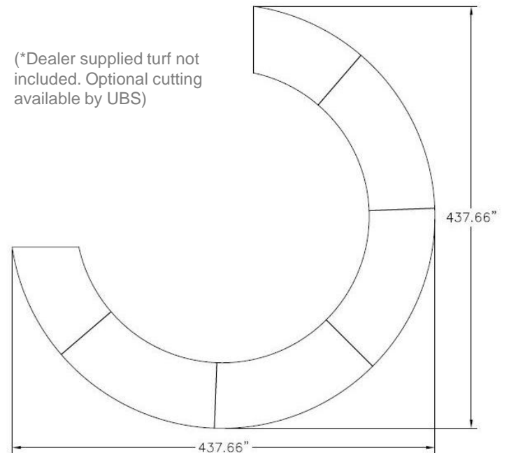
#185U 5' No Wings Turf Assembly * 03/07/12
